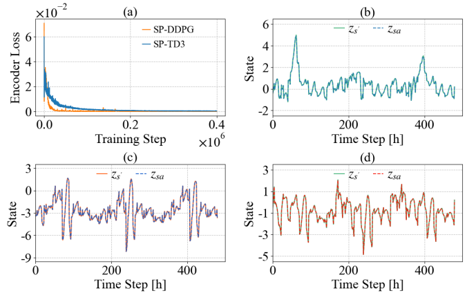
Fig. 3: Convergence of latent dynamics learning and its predictive capability.
