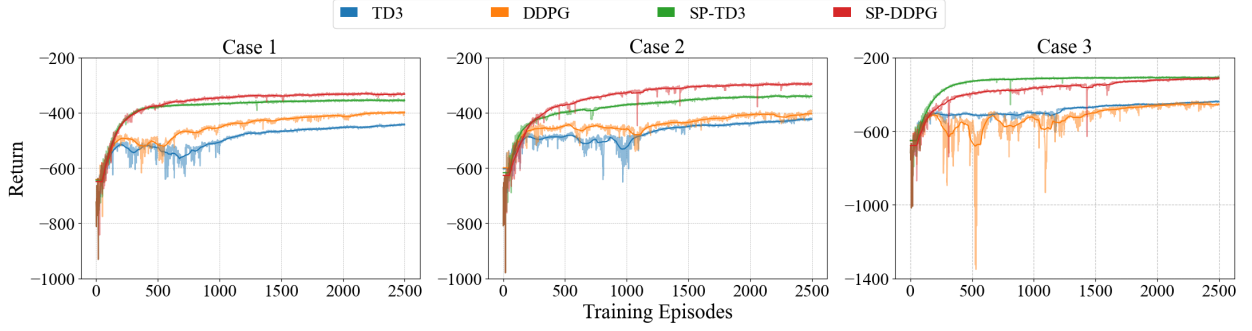
Fig. 4: The evolution of episode return during training under different methods.
