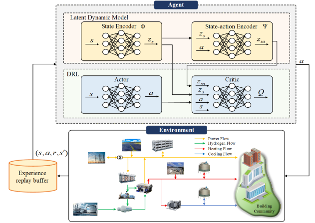
Fig. 2: The architecture of self-predictive DRL
